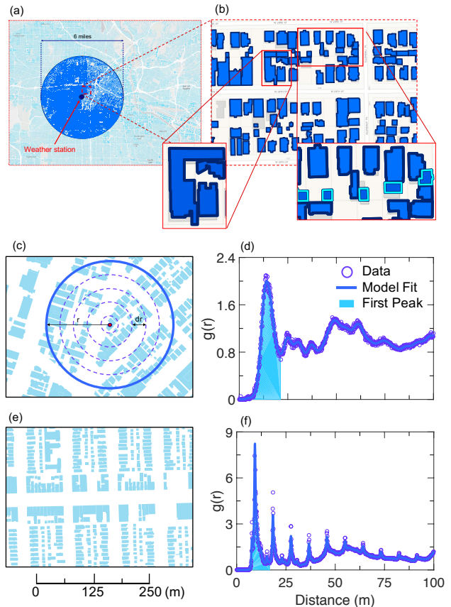
FIG. 2. (color online) Radial distribution function, g(r) , for city texture that depicts visualization of data editing, analysis and results. (a) Buildings within a 3-mile radius of an urban weather station are extracted. (b) Any buildings that share a wall are merged and any unoccupied buildings (i.e. garages) are removed from the sample of buildings transformed into a set of single points using buildings' 2-D center of mass. (c) City texture of Los Angeles, CA showing a comparable absence of order of buildings caused by dispersed streets captured by (d) the smooth and outspread peaks in g(r) , which generally are characteristic properties of liquids. (e) City texture of Chicago, IL showing order of buildings and periodicity reflected in (f) the sharp and narrow peaks of g(r) , characteristics that are known to be the hallmark of highly ordered and stable crystalline materials.
